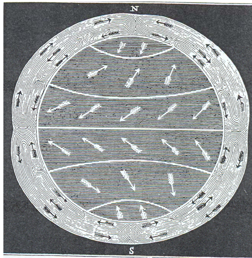
Ferrel-Thomson's circulation
