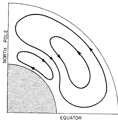
Ferrel-Thomson's circulation
