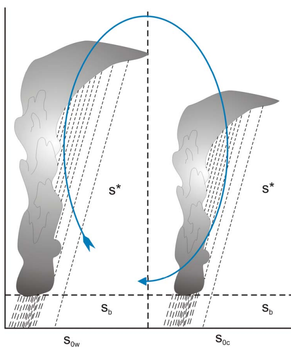
Weak circulation: Deep convection in both boxes
