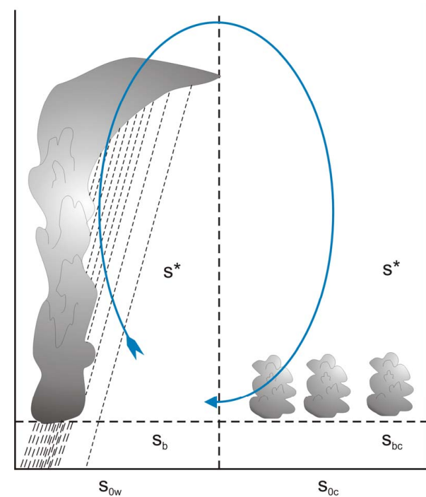
Strong circulation: Deep convection only in warm box
