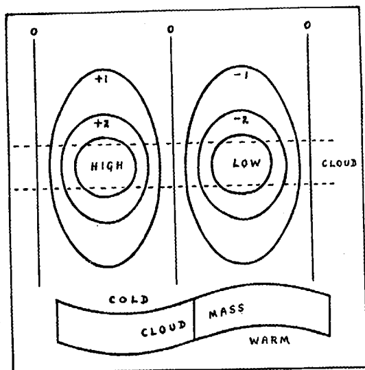
Fig. 5. Pressure-field and Cloud-mass Perturbation.
